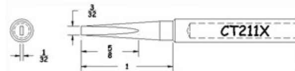
Conical Chisel
