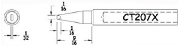
Conical Chisel
