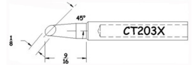
45 deg Conical Bevel
